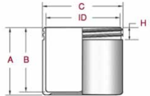
Heavy Wall Jar
