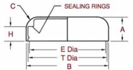
Domed Closure (Smooth or Textured)
