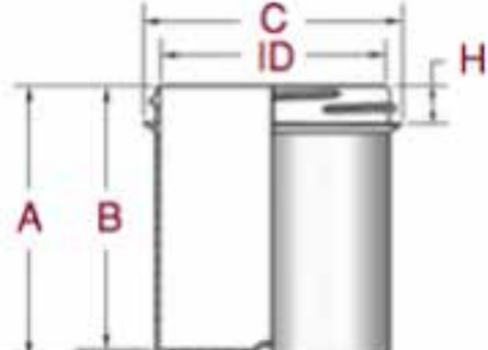
Straight Based Single Wall Jar
