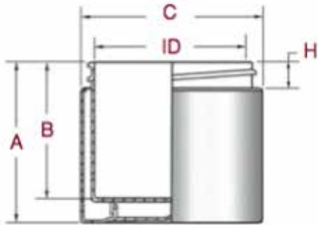
Straight Based Double Wall Jar
